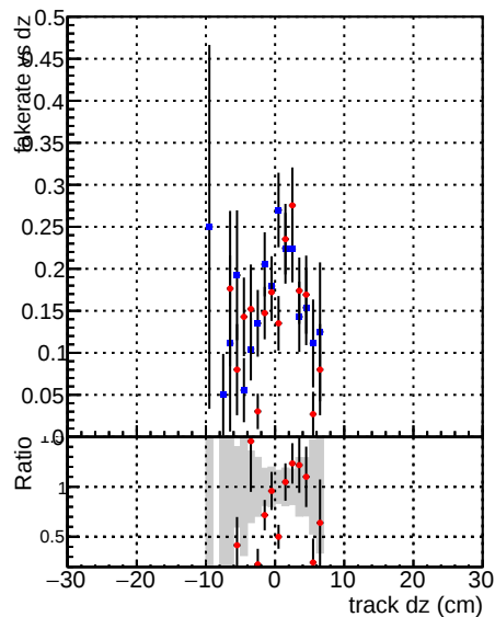
Global CMSSW_ckf RECO Fake rate vs d DQM_V0001_R0000000001 DQM_V0001_R0000000001 DQM_V0001_R0000000001 Duplicates Rate vs Dxy DQM_V0001_R0000000001 DQM_V0001_R0000000001 DQM_V0001_R0000000001 Pileup rate vs dxy DQM_V0001_R0000000001 DQM_V0001_R0000000001 DQM_V0001_R0000000001
