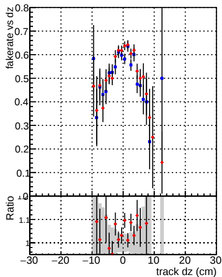
Global CMSSW_ckf_RECO Global CMSSW_mkFitOriginal_RECO DQM_V0001_R0000000001 DQM_V0001_R0000000001
