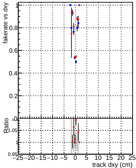
Global CMSSW_ckf_RECO Global CMSSW_mkFitOriginal_RECO DQM_V0001_R0000000001 DQM_V0001_R0000000001
