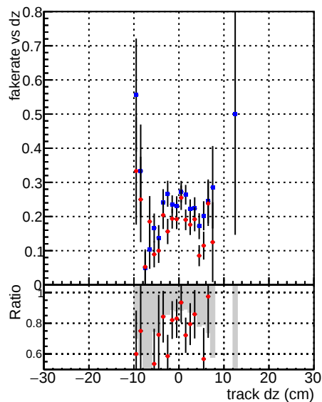
Fake rate vs dz —●— DQM_V0001_R0000000001_Global_CMSSW_ckf_RECO —●— DQM_V0001_R0000000001_Global_CMSSW_mkFitOriginal_RECO
