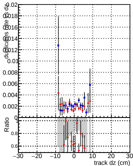
—■— DQM V0001_R000000001 Global CMSSW_ckf_RECO —●— DQM V0001_R000000001 Global CMSSW_mkFitOriginal_RECO
