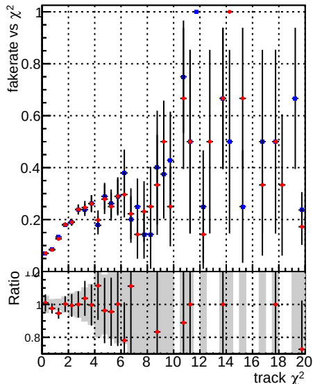
Fake rate vs. —●— DQM V0001_R000000001 Global CMSSW_ckpt_RECO —●— DQM V0001_R000000001 Global CMSSW_mkFitOriginal_RECO
