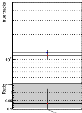
N of reco track vs. \chi^2 DQM_V0001_R000000001_Global_CMSSW_ckf_RECO DQM_V0001_R000000001_Global_CMSSW_mkFitOriginal_RECO
