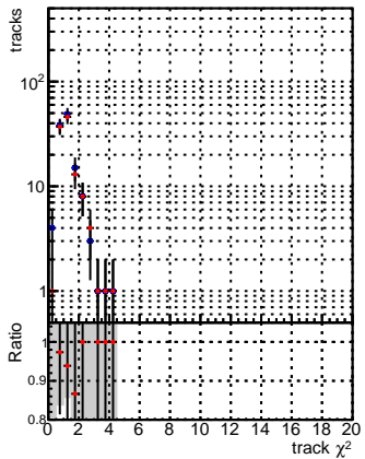
N of reco track vs. \chi^2 DQM_V0001_R000000001_Global_CMSSW_ckf_RECO DQM_V0001_R000000001_Global_CMSSW_mkFitOriginal_RECO
