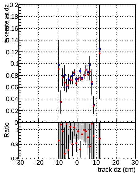
Fake rate vs dz Global CMSSW_ckf RECO DQM_V0001_R0000000001 Global CMSSW_mkFitOriginal RECO
