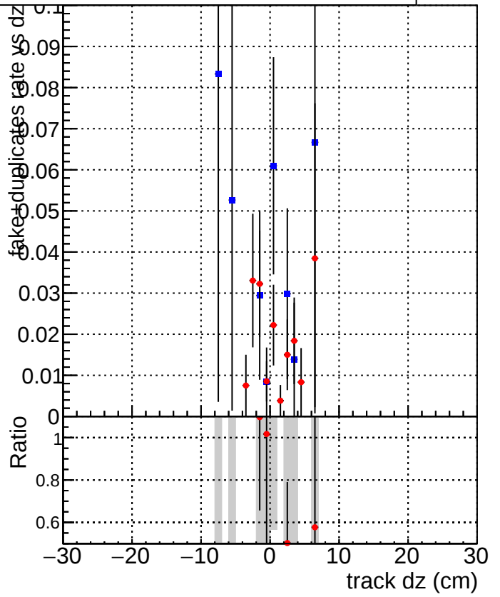
DQM_V0001_R0000000001_Global_CMSSW_ckf_RECO DQM_V0001_R0000000001_Global_CMSSW_mkFitOriginal_RECO
