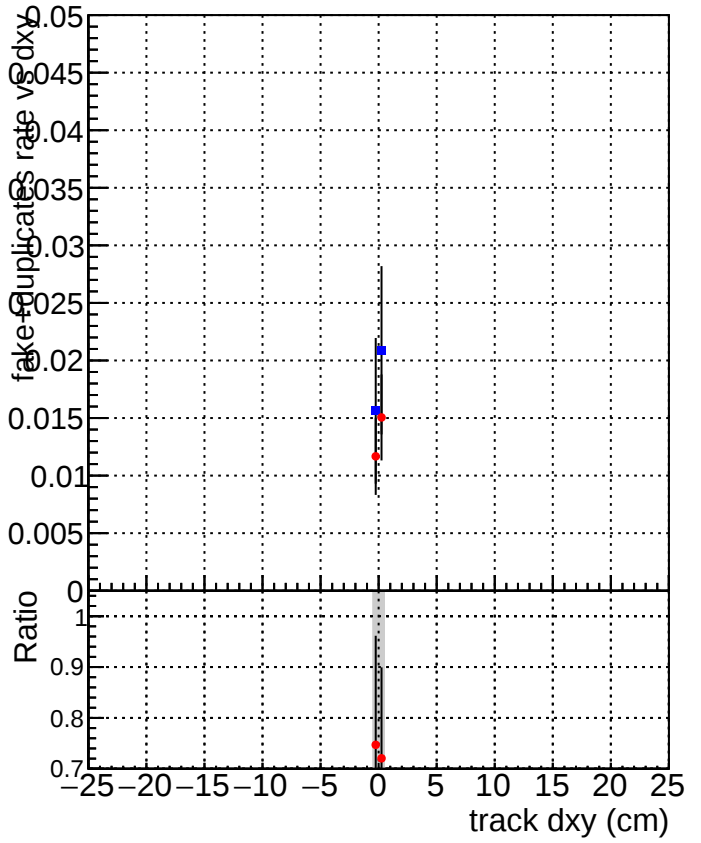
DQM_V0001_R0000000001_Global_CMSSW_ckf_RECO DQM_V0001_R0000000001_Global_CMSSW_mkFitOriginal_RECO
