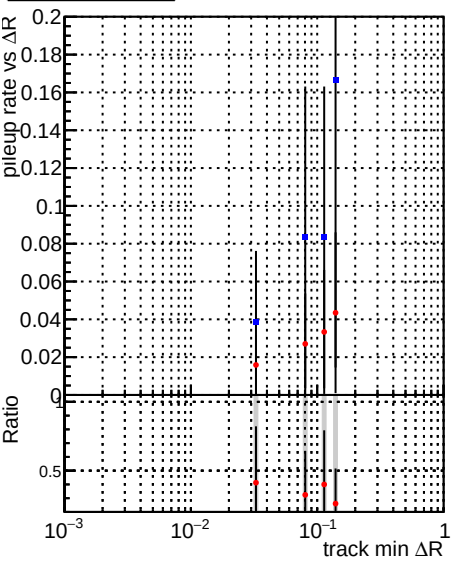
Legend: —•— DQM_V0001_R000000001_Global_CMSSW_ckf_RECO —•— DQM_V0001_R000000001_Global_CMSSW_mkFitOriginal_RECO
