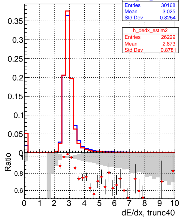
—■ DQM_V0001_R000000001_Global_CMSSW_ckf_RECO —● DQM_V0001_R000000001_Global_CMSSW_mkFitOriginal_RECO
