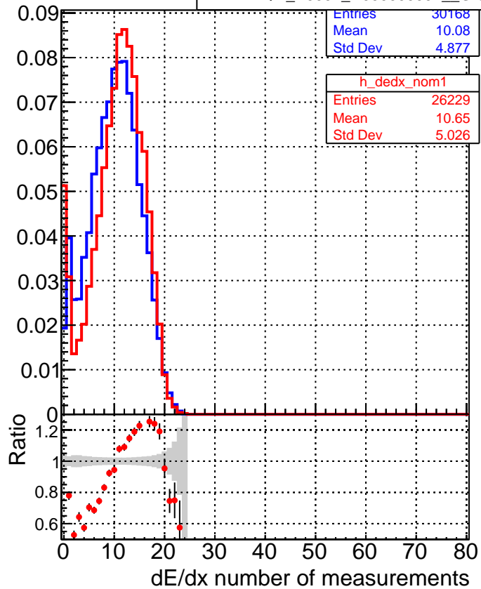
—■ DQM_V0001_R000000001_Global_CMSSW_ckf_RECO —● DQM_V0001_R000000001_Global_CMSSW_mkFitOriginal_RECO
