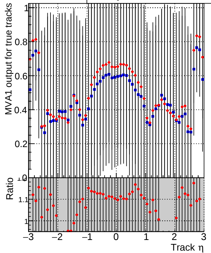
MVA1 of associated tracks (recoToSim) vs. track \eta Legend: ■ DQM_V0001_R000000001_Global_CMSSW_ckf_RECO ■ DQM_V0001_R000000001_Global_CMSSW_mkFitOriginal_RECO
