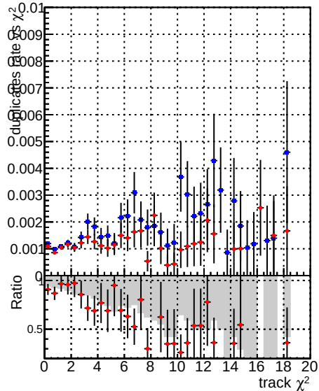
—●— DQM_V0001_R0000000001_Global_CMSSW_ckf_RECO —●— DQM_V0001_R0000000001_Global_CMSSW_mkFitOriginal_RECO
