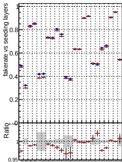
—●— DQM_V0001_R0000000001_Global_CMSSW_ckf_RECO —●— DQM_V0001_R0000000001_Global_CMSSW_mkFitOriginal_RECO
