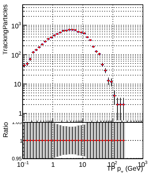
Legend: DQM_V0001_R000000001_Global_CMSSW_ckf_RECO (blue squares), DQM_V0001_R000000001_Global_CMSSW_mkFitOriginal_RECO (red diamonds)
