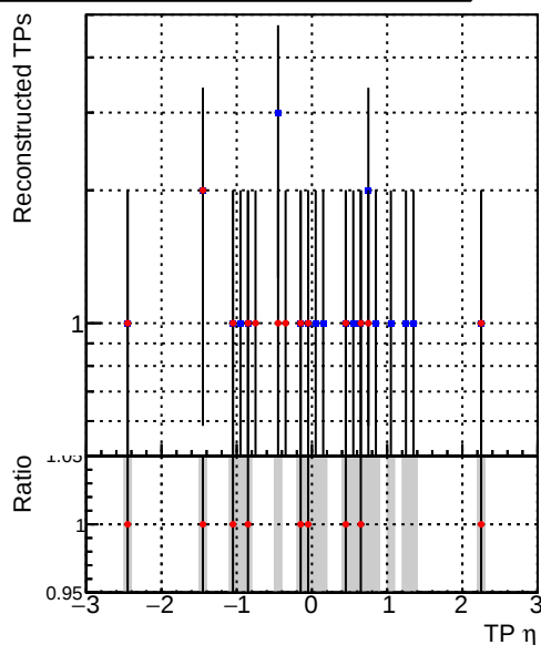
Legend: DQM_V0001_R000000001_Global_CMSSW_ckf_RECO (blue squares), DQM_V0001_R000000001_Global_CMSSW_mkFitOriginal_RECO (red diamonds)
