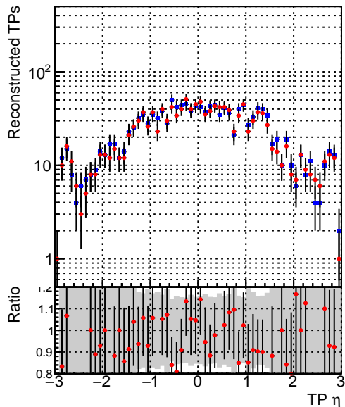
—●— DQM_V0001_R0000000001_Global_CMSSW_ckf_RECO —●— DQM_V0001_R0000000001_Global_CMSSW_mkFitOriginal_RECO
