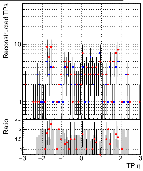
N of simulated tracks vs \eta Legend: — DQM_V0001_R000000001_Global_CMSSW_ckf_RECO (blue line) — DQM_V0001_R000000001_Global_CMSSW_mkFitOriginal_RECO (red line)
