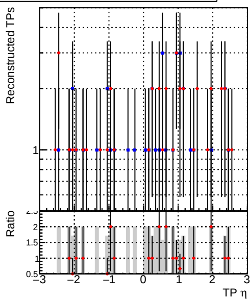
Legend: DQM_V0001_R000000001_Global_CMSSW_ckf_RECO (blue diamonds), DQM_V0001_R000000001_Global_CMSSW_mkFitOriginal_RECO (red diamonds)
