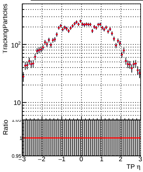
Legend: DQM_V0001_R000000001_Global_CMSSW_ckf_RECO (blue line with error bars), DQM_V0001_R000000001_Global_CMSSW_mkFitOriginal_RECO (red line with error bars)
