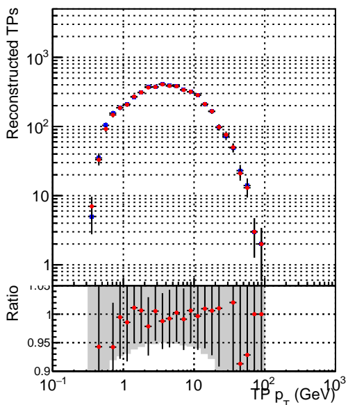
— DQM_V0001_R0000000001_Global_CMSSW_ckf_RECO — DQM_V0001_R0000000001_Global_CMSSW_mkFitOriginal_RECO
