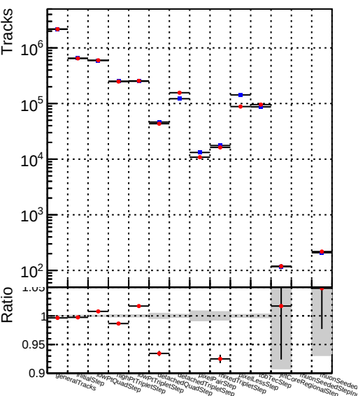
DQM_V0001_R000000001_Global_CMSSW_ckf_RECO
