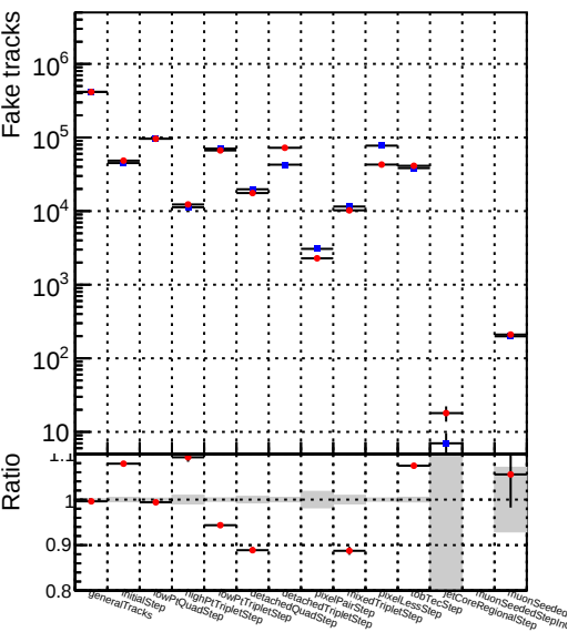
Numbe —●— DQM_V0001_R000000001_Global_CMSSW_mkFitOriginal_RECO
