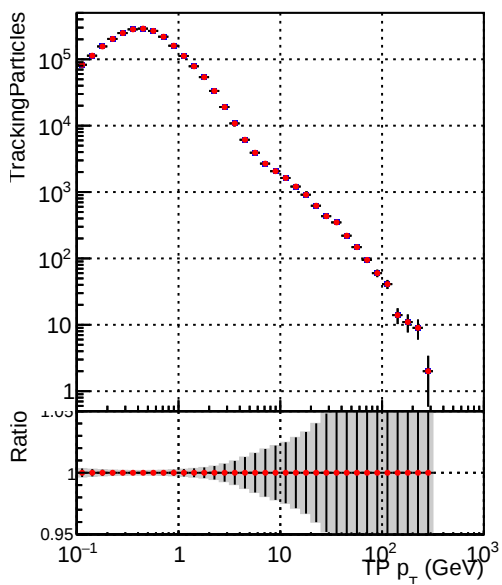
■ DQM_V0001_R0000000001_Global_CMSSW_ckf_RECO ■ DQM_V0001_R0000000001_Global_CMSSW_mkFitOriginal_RECO
