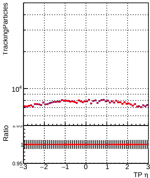
■ DQM_V0001_R0000000001_Global_CMSSW_ckf_RECO ■ DQM_V0001_R0000000001_Global_CMSSW_mkFitOriginal_RECO
