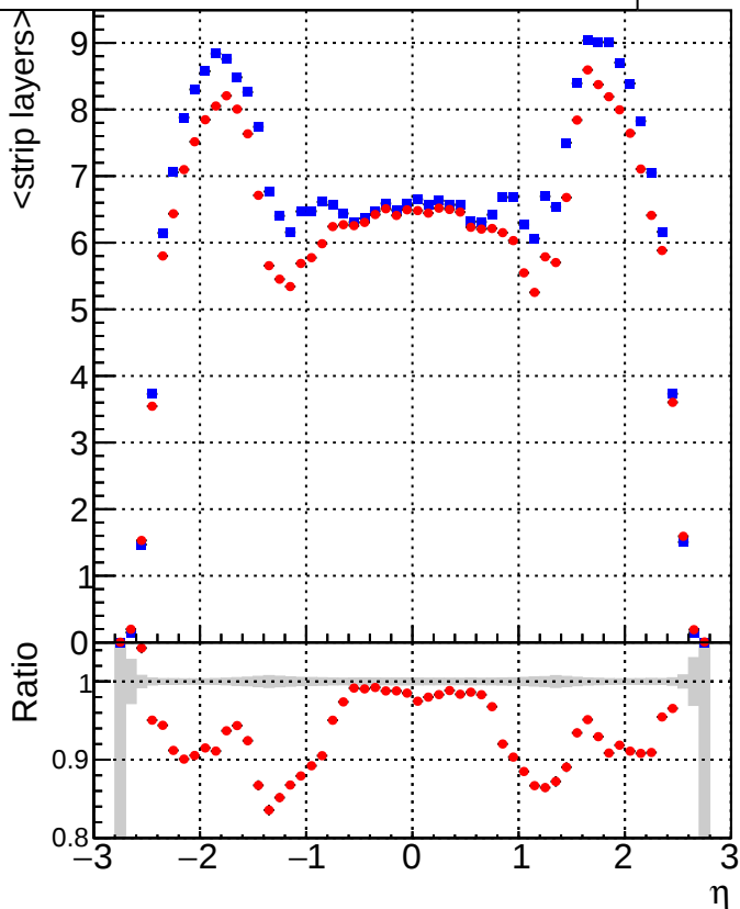
Legend: DQM_V0001_R000000001_Global_CMSSW_ckf_RECO DQM_V0001_R000000001_Global_CMSSW_mkFitOriginal_RECO
