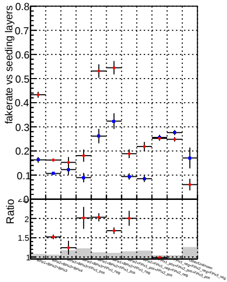
Fake rate vs. —•— DQM_V0001_R000000001_Global_CMSSW_ckf_RECO —•— DQM_V0001_R000000001_Global_CMSSW_mkFitOriginal_RECO
