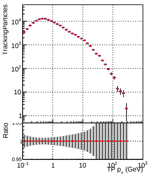
—•— DQM_V0001_R000000001_Global_CMSSW_ckf_RECO —•— DQM_V0001_R000000001_Global_CMSSW_mkFitOriginal_RECO
