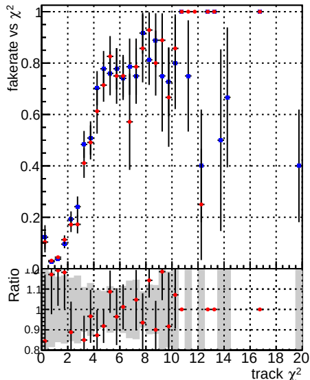
Fake rate vs. —●— DQM V0001_R000000001 Global CMSSW_ckf_RECO —●— DQM V0001_R000000001 Global CMSSW_mkFitOriginal_RECO
