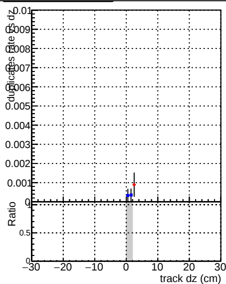
—■— DQM_V0001_R0000000001 Global_CMSSW_ckf_RECO —●— DQM_V0001_R0000000001 Global_CMSSW_mkFitOriginal_RECO
