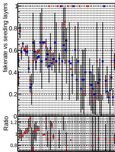
Fake rate vs. Legend: Blue circle: DQM V0001_R000000001_Global_CMSSW_ckf_RECO Red circle: DQM V0001_R000000001_Global_CMSSW_mkFitOriginal_RECO
