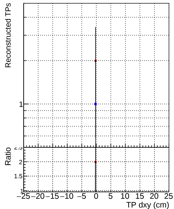
N of simulated track ■ DQM_V0001_R000000001 Global CMSSW_ckfnocut3_RECO ● DQM_V0001_R000000001 Global CMSSW_mknocut3_RECO ▲ DQM_V0001_R000000001 Global CMSSW_mknocutinoclean3_RECO
