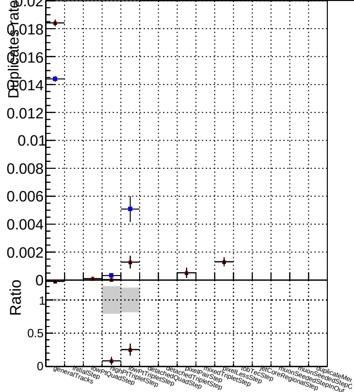
Duplicates rate vs collection ■ DQM V0001_R000000001 Global CMSSW ckfnocut3 RECO ● DQM V0001_R000000001 Global CMSSW mknocut3 RECO ▲ DQM V0001_R000000001 Global CMSSW mknocut3 RECO
