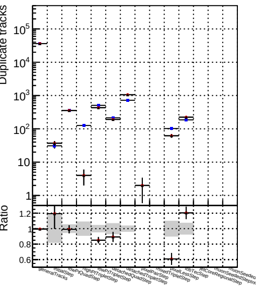
Number Legend Label Scope Variable DQM_V0001_R0000000001 Global CMSSW_ckfnocut3_RECO DQM_V0001_R0000000001 Global CMSSW_mknocut3_RECO DQM_V0001_R0000000001 Global CMSSW_mknocutnucleon3_RECO
