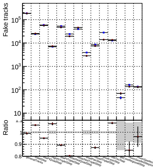
Number of tracks vs collection DQM_V0001_R000000001_Global_CMSSW_ckfnocut3_RECO DQM_V0001_R000000001_Global_CMSSW_mknocut3_RECO DQM_V0001_R000000001_Global_CMSSW_mknocutinoclean3_RECO
