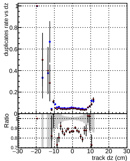
Legend for all plots: DOM V0001 (blue line) DOM V0001 R0000000001 (red line) Global (black line) CMSSW ckmocut3 RECO (grey shaded area) CMSSW mknocut3 RECO (light grey shaded area) CMSSW mknocut3clean3 RECO (dark grey shaded area)
