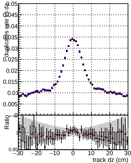
Global CMSSW cknocut3 RECO
