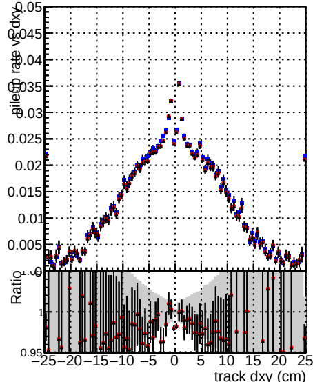
Global CMSSW mknocut3 RECO
