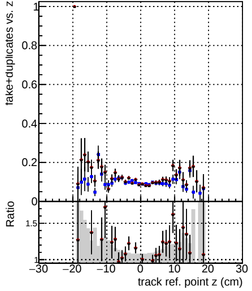
—●— DQM_V0001_R0000000001_Global_CMSSW_cknocut3_RECO —●— DQM_V0001_R0000000001_Global_CMSSW_mknocut3_RECO —●— DQM_V0001_R0000000001_Global_CMSSW_mknocutinoclean3_RECO
