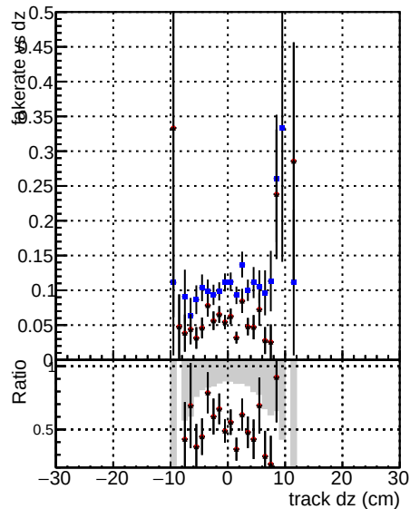
Fake rate vs d DOM V0001 DOM V0001 Global CMSSW cknocut3 RECO DOM V0001 DOM V0001 Global CMSSW mknocut3 RECO DOM V0001 DOM V0001 Global CMSSW mknocut3clean3 RECO
