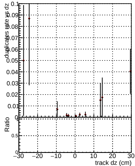
a|---CMSSW_mknocut3_RE a|---CMSSW_mknocutinocl
