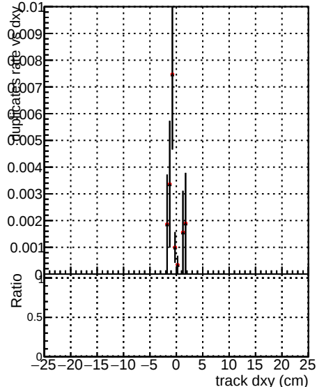
a|---CMSSW_mknocut3_RE a|---CMSSW_mknocutinocl
