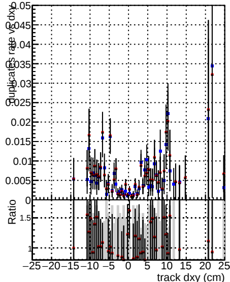
DOM V0001 R0000000001 Global CMSSW ckfncut3 RECO DOM V0001 R0000000001 Global CMSSW mknocut3 RECO DOM V0001 R0000000001 Global CMSSW mknocut3clean3 RECO
