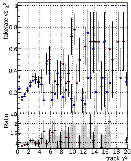
Fake rate vs. DOM_V0001 R0000000001 Global CMSSW_ckfnocut3_RECO DOM_V0001 R0000000001 Global CMSSW_mknocut3_RECO DOM_V0001 R0000000001 Global CMSSW_mknocut3clean3_RECO
