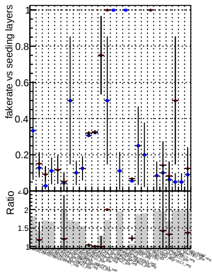
Fake rate vs. DOM_V0001 R0000000001 Global CMSSW_ckfnocut3_RECO DOM_V0001 R0000000001 Global CMSSW_mknocut3_RECO DOM_V0001 R0000000001 Global CMSSW_mknocut3clean3_RECO
