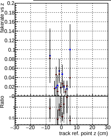
Legend: - Global CMSSW_ckfnocut3_RECO - Global CMSSW_mknocut3_RECO - Global CMSSW_mknocutinoclean3_RECO
