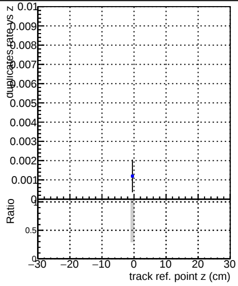
—●— DQM_V0001_R0000000001_Global_CMSSW_ckfnocut3_RECO —●— DQM_V0001_R0000000001_Global_CMSSW_mknocut3_RECO —●— DQM_V0001_R0000000001_Global_CMSSW_mknocutinoclean3_RECO
