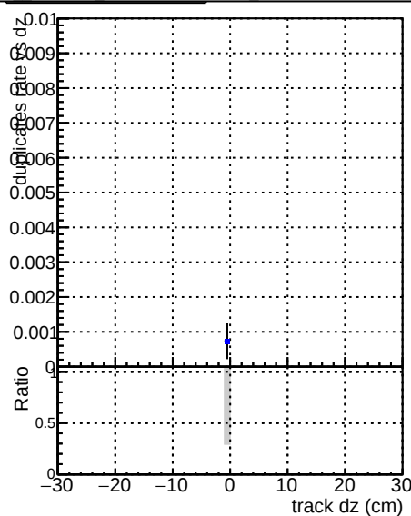
DOM V0001 R0000000001 Global CMSSW_ckmcut3 RECO DOM V0001 R0000000001 Global CMSSW_mknocut3 RECO DOM V0001 R0000000001 Global CMSSW_mknocut3clean3 RECO
