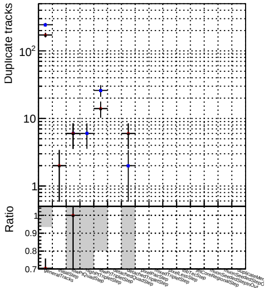
—●— DQM_V0001_R000000001_Global_CMSSW_cknocut3_RECO —●— DQM_V0001_R000000001_Global_CMSSW_mknocut3_RECO —●— DQM_V0001_R000000001_Global_CMSSW_mknocutinoclean3_RECO
