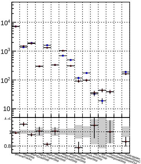
—●— DQM_V0001_R000000001_Global_CMSSW_cknocut3_RECO —●— DQM_V0001_R000000001_Global_CMSSW_mknocut3_RECO —●— DQM_V0001_R000000001_Global_CMSSW_mknocutinoclean3_RECO
