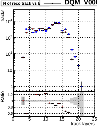
N of reco track vs layer
