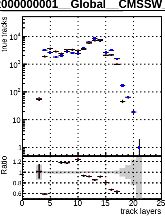
N of associated (recoToSim) tracks vs layer
