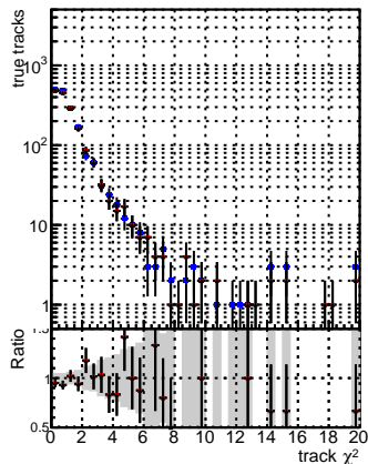
1 G oba C M S S W m knocut3 RECO G oba C M S S W m knocut3noclean3 RECO
