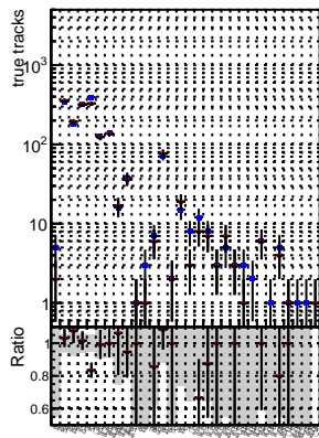
1 G oba C M S S W m knocut3 RECO G oba C M S S W m knocut3noclean3 RECO
