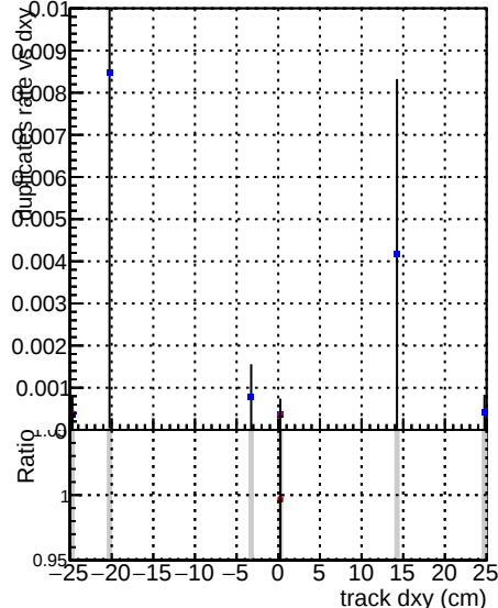
Global CMSSW cknocut3 RECO Global CMSSW mknocut3 RECO
