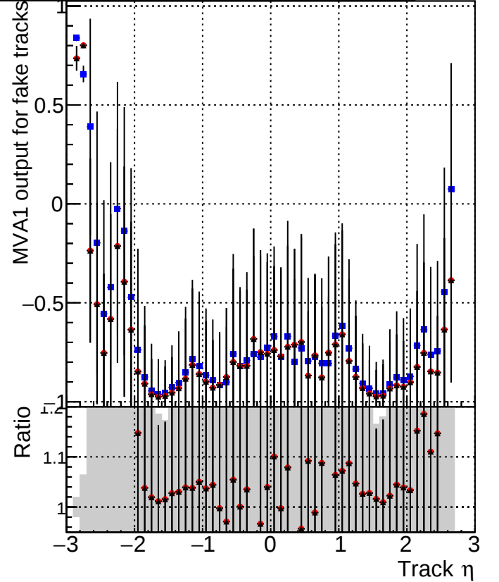
MVA1 of associated tracks (recoToSim) vs. track \eta ■ DQM_V0001_R000000001_Global_CMSSW_ckfnocut3_RECO ● DQM_V0001_R000000001_Global_CMSSW_mknocut3_RECO ▲ DQM_V0001_R000000001_Global_CMSSW_mknocutinoclean3_RECO
