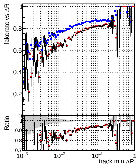
—●— DQM_V0001_R000000001 Global CMSSW_ckfnocut3_RECO —●— DQM_V0001_R000000001 Global CMSSW_mknocut3_RECO —●— DQM_V0001_R000000001 Global CMSSW_mknocut3clean3_RECO
