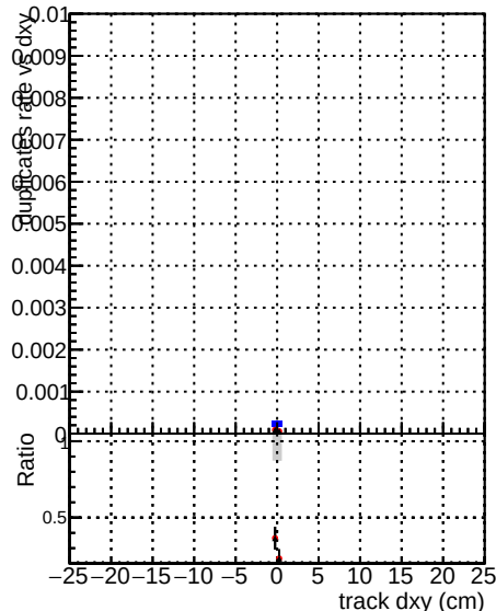
DOM V0001 DOM V0001 Global CMSSW ckmocut3 RECO DOM V0001 DOM V0001 Global CMSSW mknocut3 RECO DOM V0001 DOM V0001 Global CMSSW mknocut3clean3 RECO
