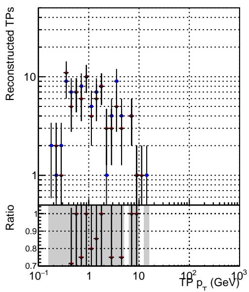
—●— DQM_V0001_R000000001 Global_CMSSW_ckfnocut3_RECO —●— DQM_V0001_R000000001 Global_CMSSW_mknocut3_RECO —●— DQM_V0001_R000000001 Global_CMSSW_mknocutinoclean3_RECO
