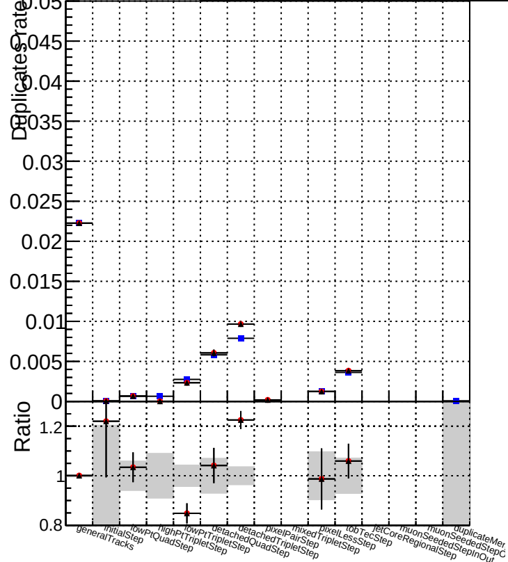
Duplicates rate vs collection Legend: DQM V0001_R000000001 Global CMSSW cknocut3 RECO DQM V0001_R000000001 Global CMSSW mknocut3 RECO DQM V0001_R000000001 Global CMSSW mknocutinoclean3 RECO
