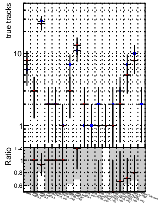
N of reco track vs. s Global CMSSW_43mcut3 RECO DCM_V0001_R0000000001 Global CMSSW_mknocut3 RECO DCM_V0001_R0000000000 Global CMSSW_mknocut3clean3 RECO
